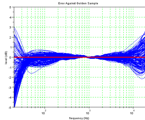
Figure 4 - Error against golden sample
