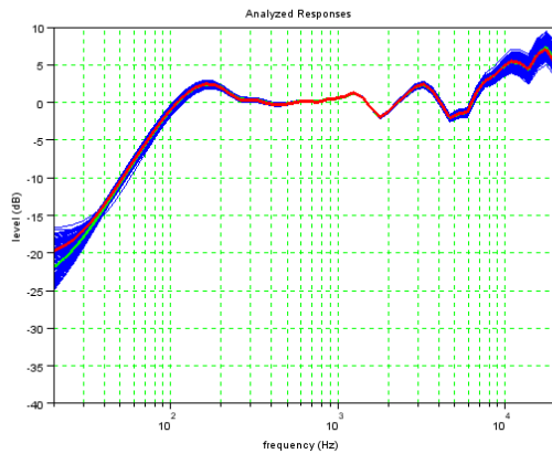
Figure 3 - (red) Golden sample response, (cyan) average response, (blue) batch responses
