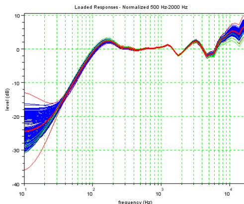
Figure 2 - Loaded responses: (red bold) Average; (red thin) Avg. +/- 3 std. deviation, (green) Outliers
