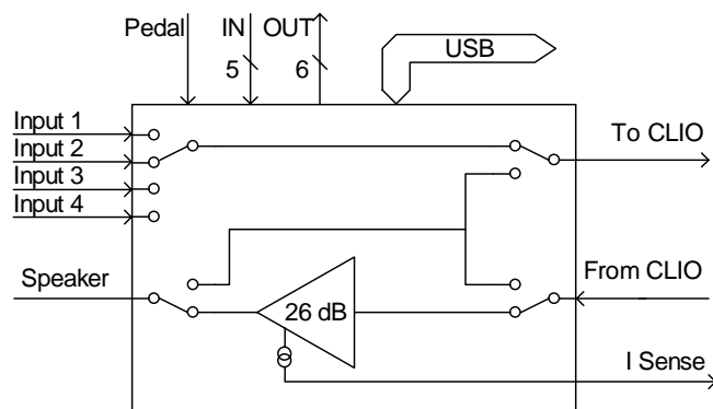
Internal connections for frequency response measurements
