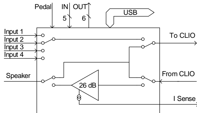
Internal connections for impedance measurements (Internal Mode)
