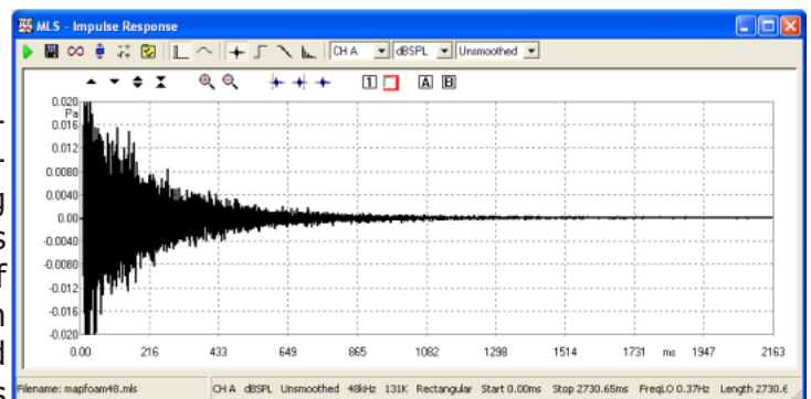
Impulse response
