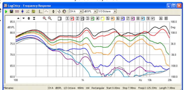
Frequency response
