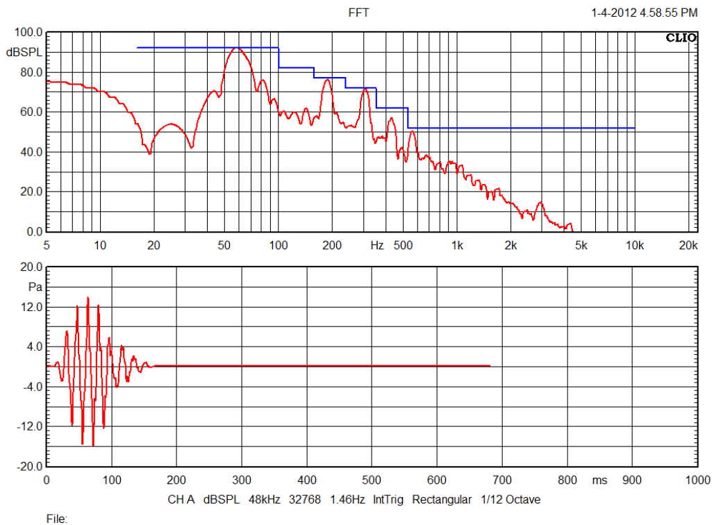
Figure 14: ACE-bass B2-50 - ANSI/CEA-2010 test @ 63 Hz
