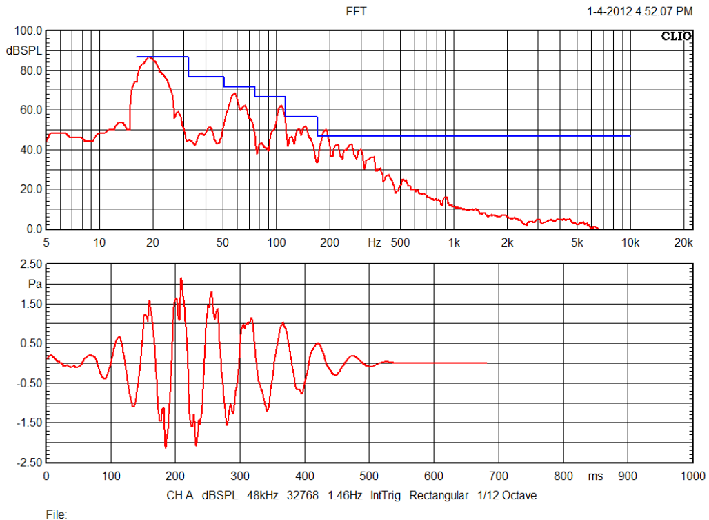
Figure 9: ACE-bass B2-50 - ANSI/CEA-2010 test @ 20 Hz
