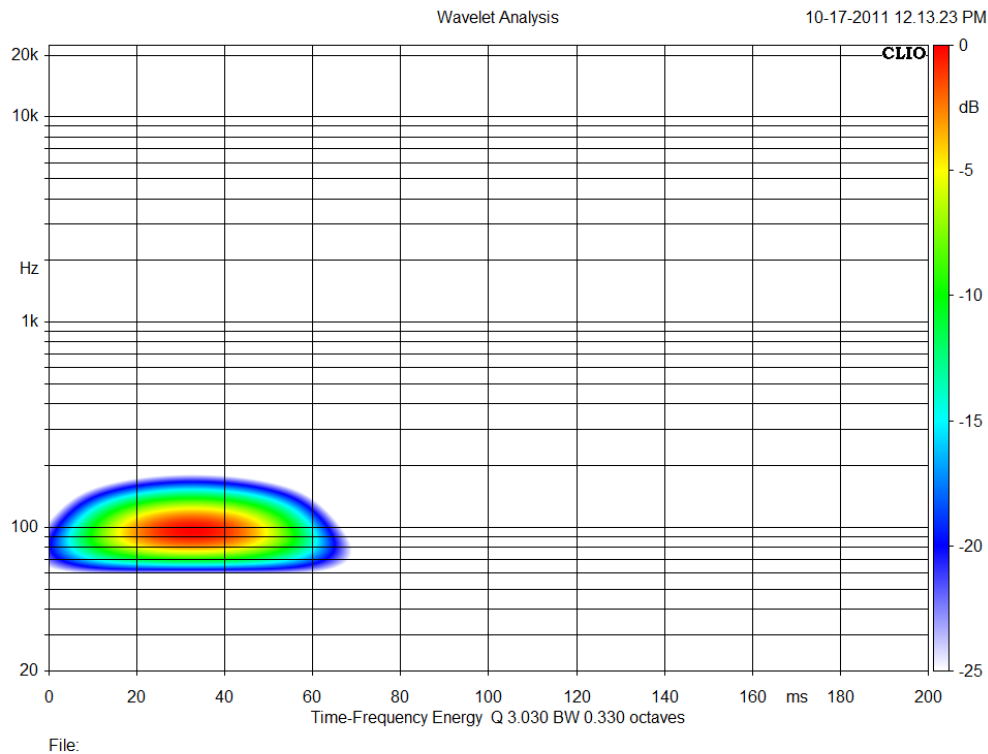
Figure 2: Joint time-frequency analysis (wavelet) of a 6.5 cycles 100 Hz hann-burst
