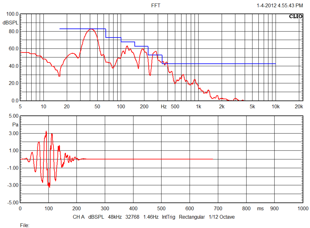
Figure 12: ACE-bass B2-50 - ANSI/CEA-2010 test @ 40 Hz
