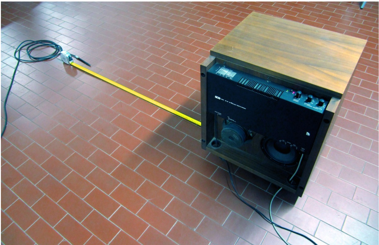
Figure 6: Tested subwoofer with microphone in ground plane configuration
