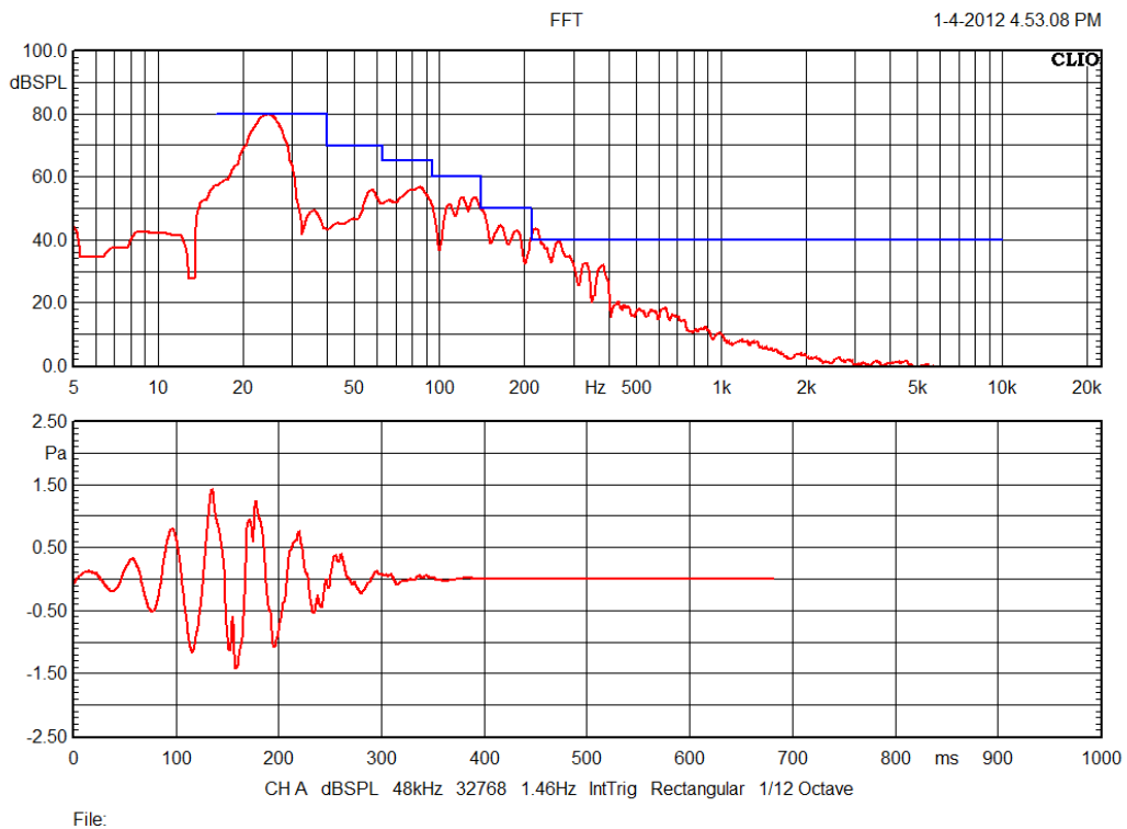
Figure 10: ACE-bass B2-50 - ANSI/CEA-2010 test @ 25 Hz
