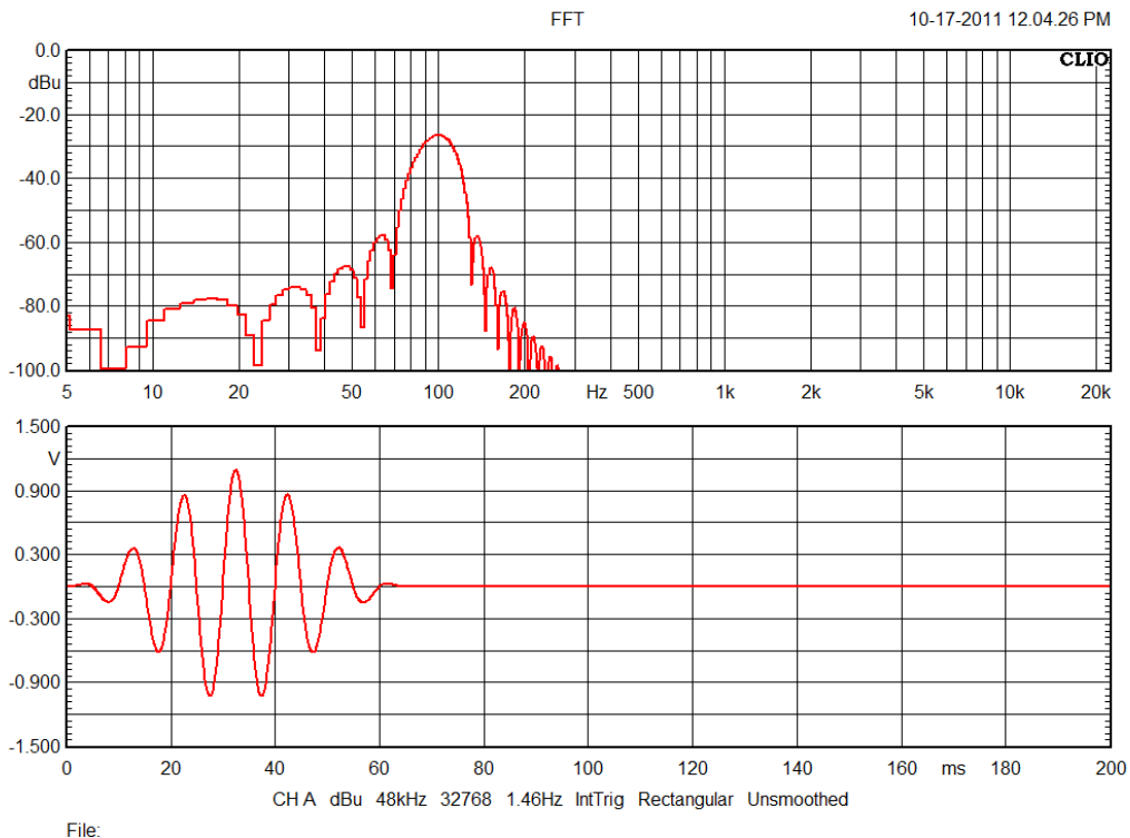
Figure 1: Waveform and magnitude spectrum of a 6.5 cycles 100 Hz hann-burst
