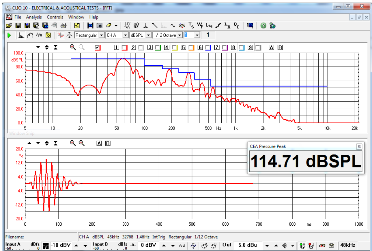
Figure 8: CLIO 10 running ANSI/CEA-2010 test
