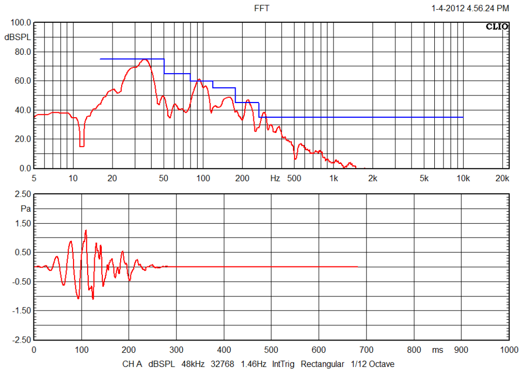
Figure 11: ACE-bass B2-50 - ANSI/CEA-2010 test @ 31.5 Hz
