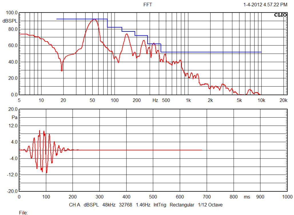
Figure 13: ACE-bass B2-50 - ANSI/CEA-2010 test @ 50 Hz
